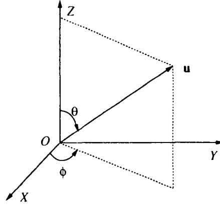
Fig. 4: Spherical coordinates
