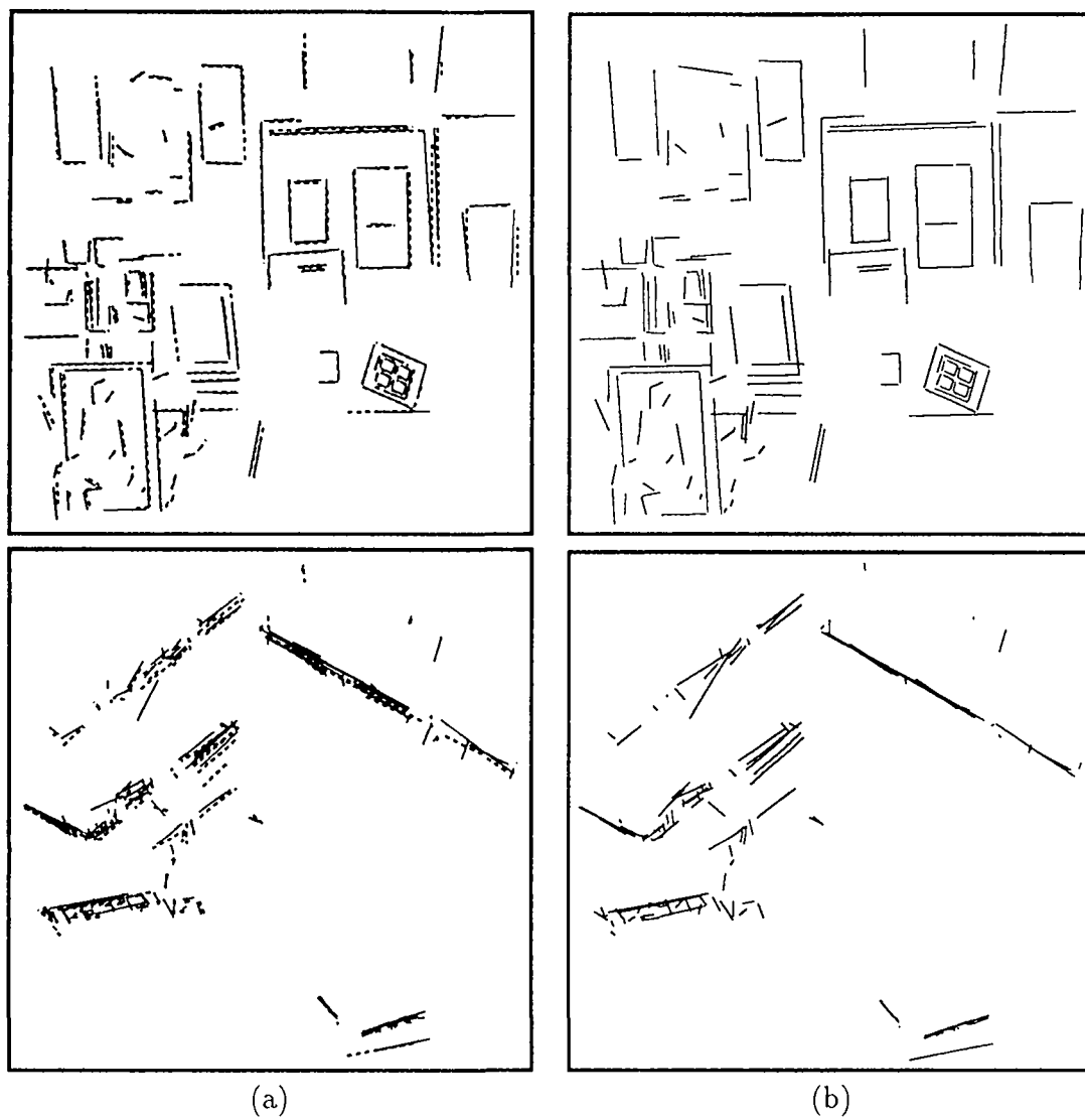
Fig. 16: (a) superposition of the matched segments after applying the estimated motion to the first frame, (b) fused segments (unmatched segments are not displayed)
