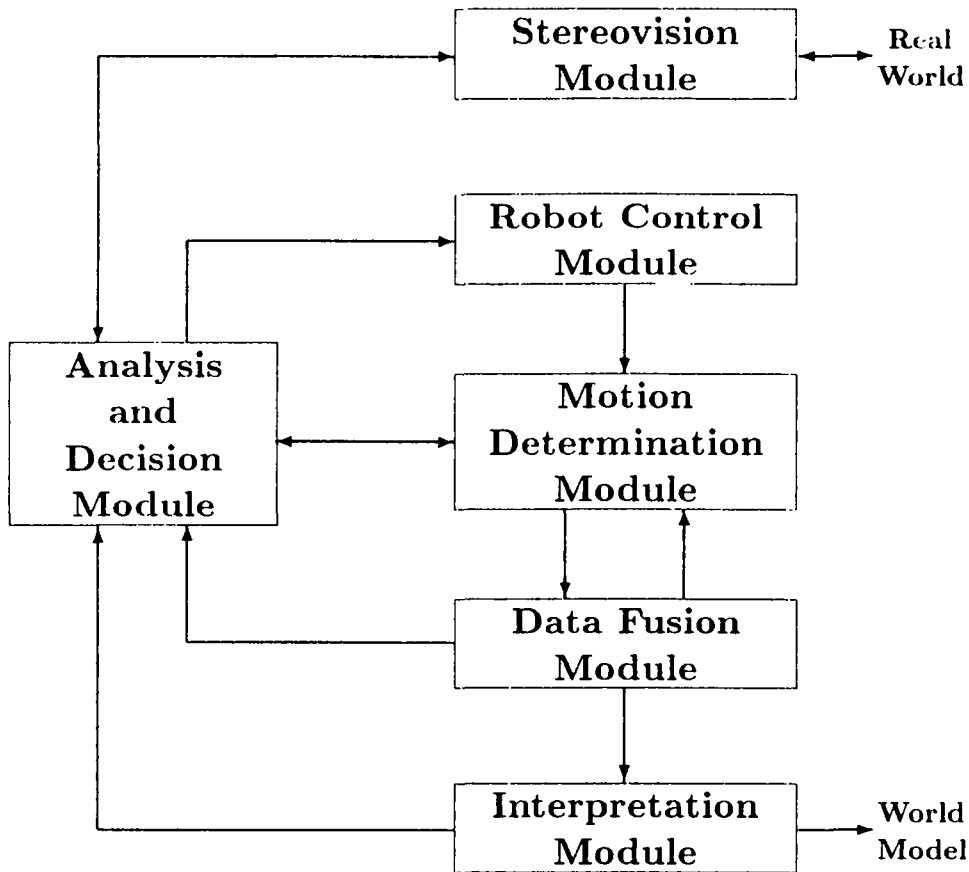
Fig. 2: System architecture
